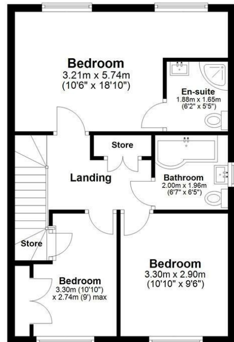
First Floor Approx. 50.0 sq. metres (538.1 sq. feet)
